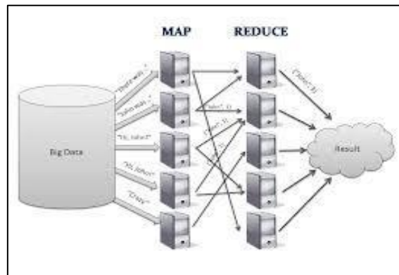
Fig 1.3: MapReduce
